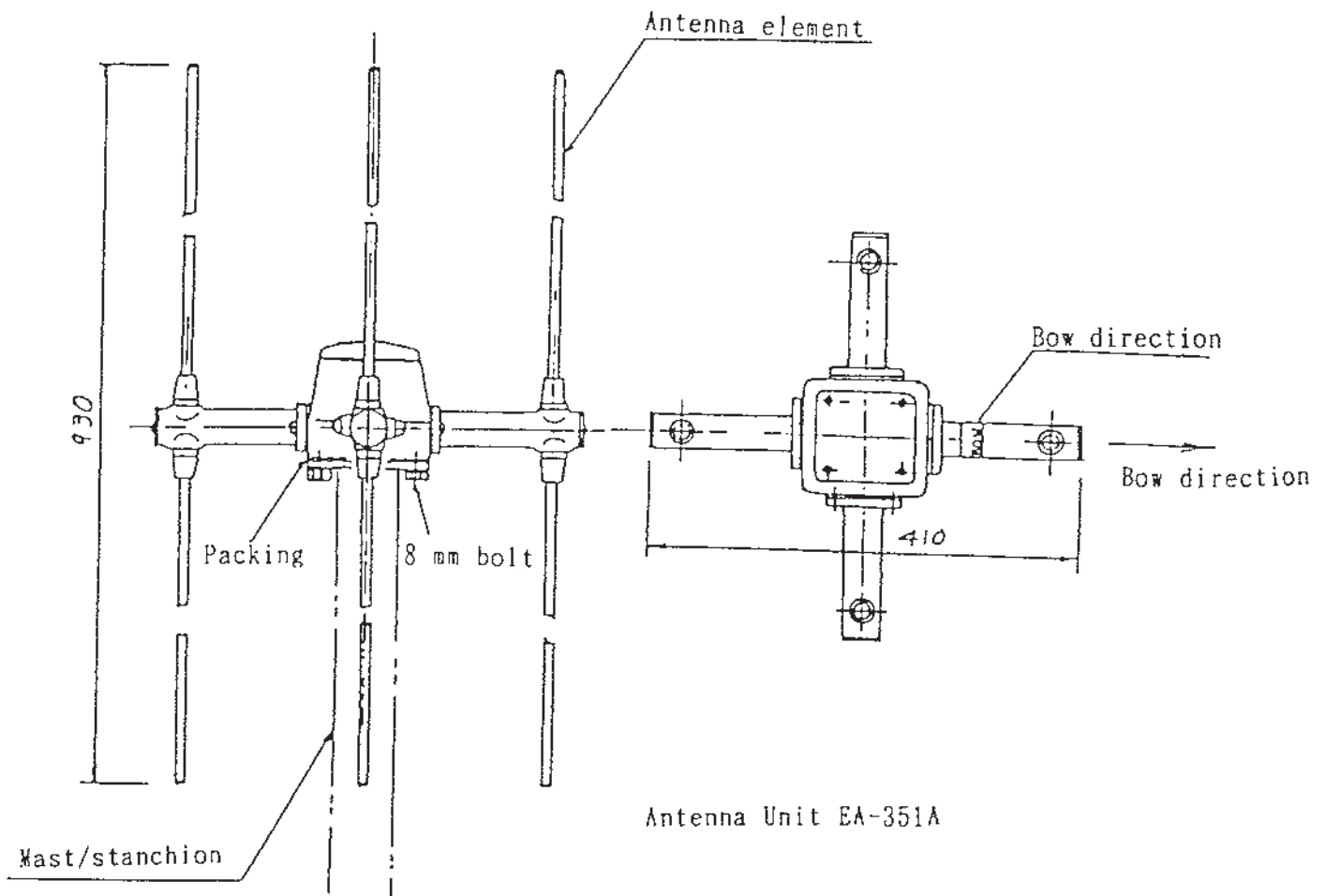
Diagram 3 Antenna Unit
